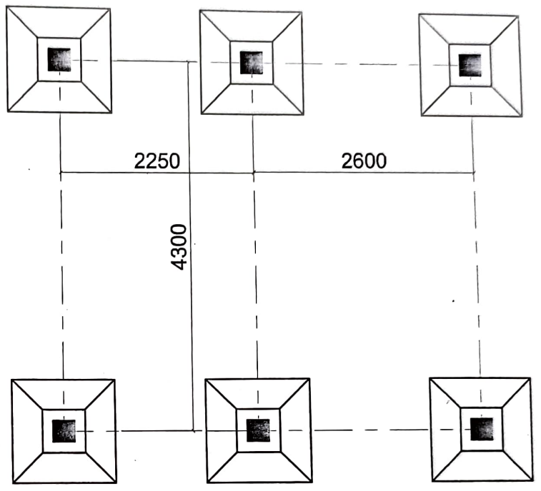
COLUMN LAYOUT PLAN
