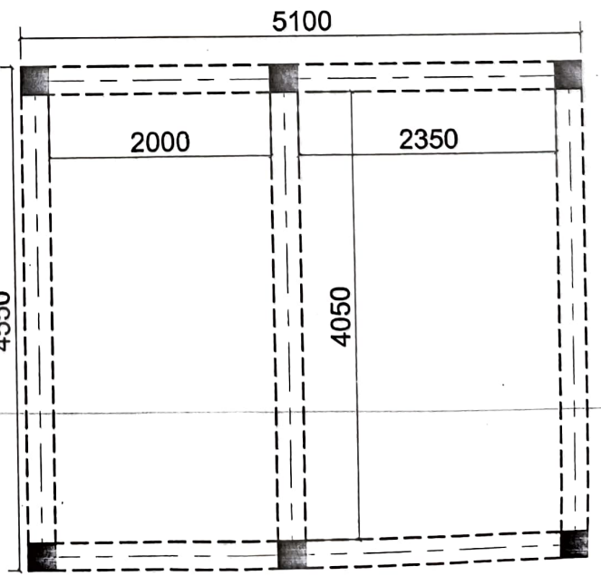
TIE & FLOOR BEAM PLAN
