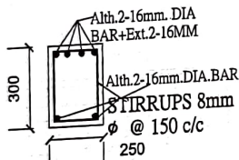
AT SUPPORT SEC. ON SLAB BEAM SCALE 1:25
