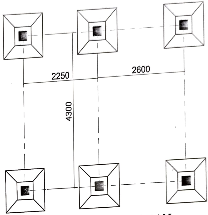
COLUMN LAYOUT PLAN
