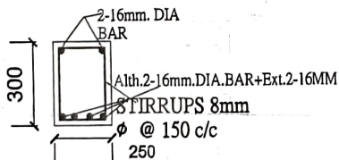
AT MID SPAN SEC. ON SLAB BEAM SCALE 1:25
