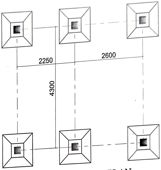
COLUMN LAYOUT PLAN COLUMN 250x250
