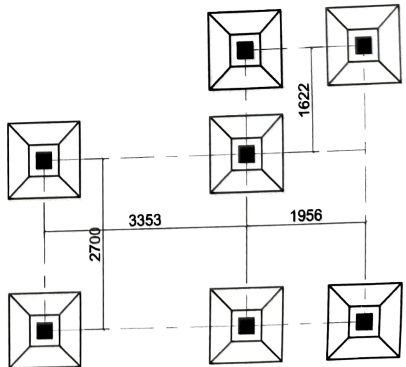
COLUMN LAYOUT PLAN COLUMN 250x250
