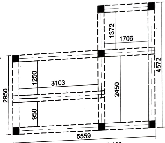
TIE & FLOOR BEAM PLAN
