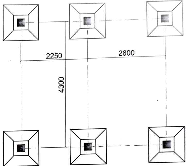
COLUMN LAYOUT PLAN COLUMN 250x250
