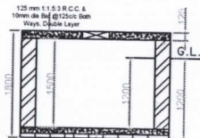
Under Ground Reservoir Details
