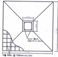
DETAILS OF FOUNDATION (SCALE 1:25)
