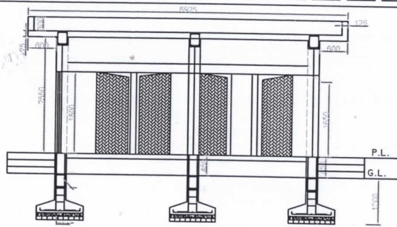
DETAILS OF WALL SECTION A-A
