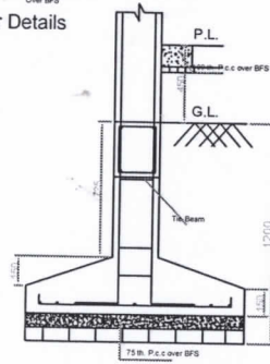
DETAILS OF FOUNDATION (SCALE 1:25)
