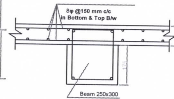
Slab Beam Details
