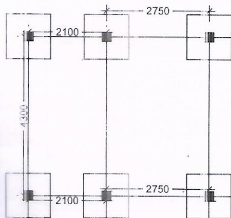
LAYOUT PLAN
