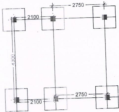
LAYOUT PLAN
