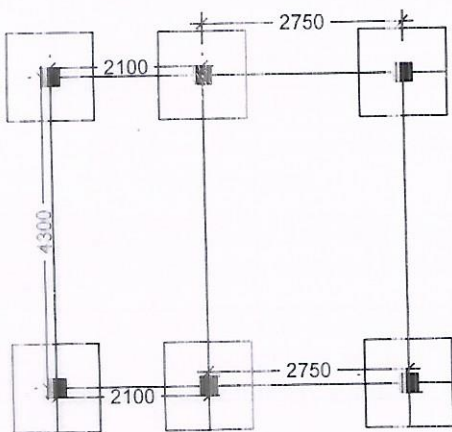
LAYOUT PLAN
