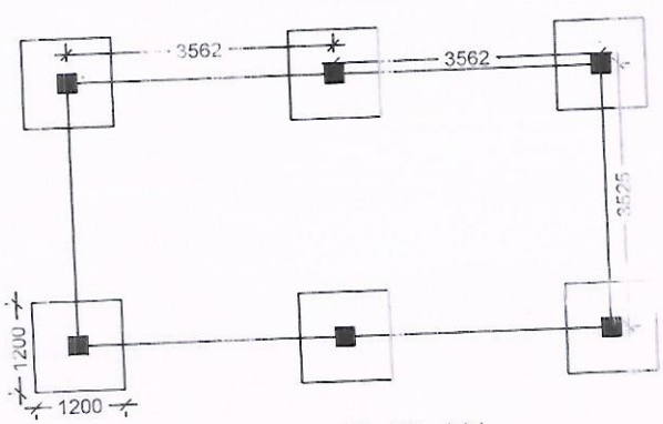
LAYOUT PLAN
