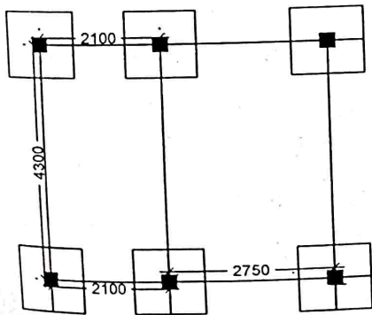
LAYOUT PLAN
