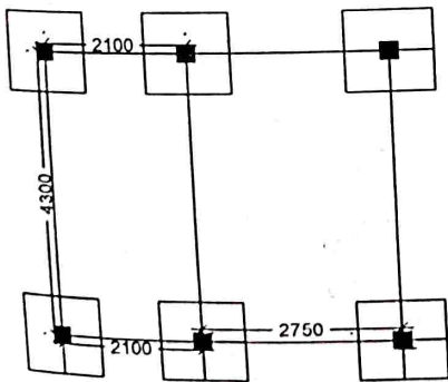
LAYOUT PLAN
