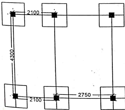
LAYOUT PLAN
