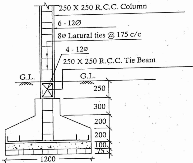
DETAILS OF R. C. C COLUMN (SCALE - 1 : 25)
