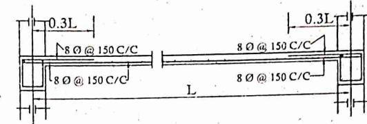
Details Of R. C. C Roof Slab & Beam (SCALE - 1 : 25)
