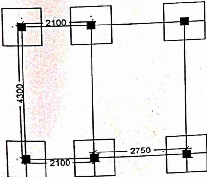
LAYOUT PLAN
