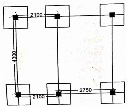
LAYOUT PLAN
