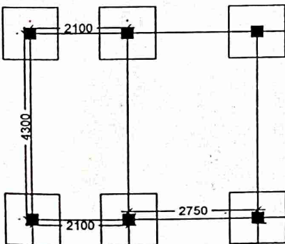
LAYOUT PLAN
