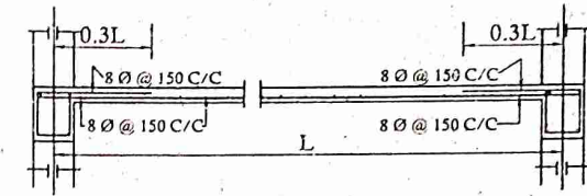
Details Of R. C. C Roof Slab & Beam
