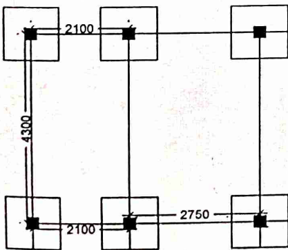
LAYOUT PLAN
