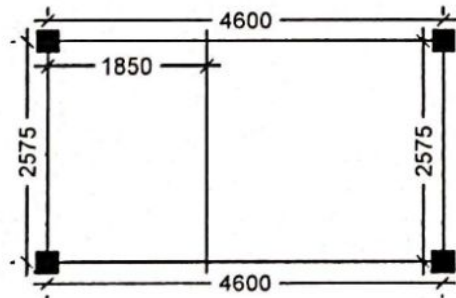
LAYOUT PLAN
