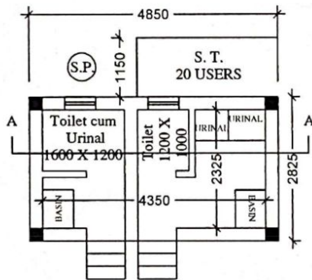
PLAN
