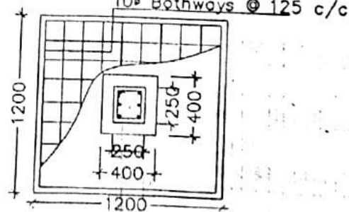
DETAILS OF R. C. C COLUMN (SCALE - 1 : 25)
