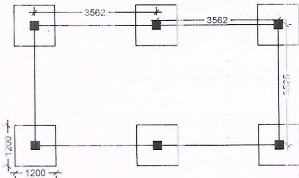
LAYOUT PLAN
