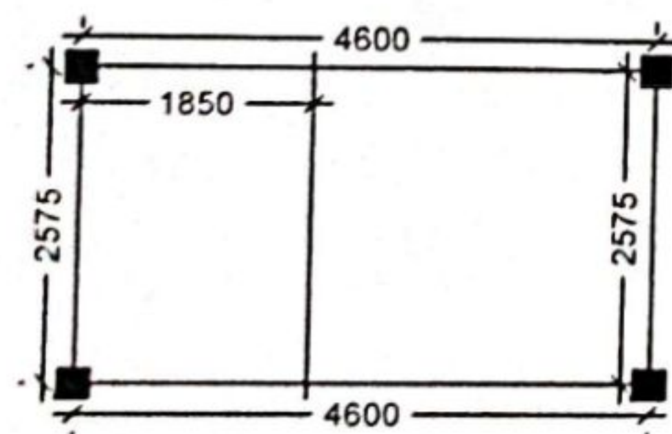
LAYOUT PLAN
