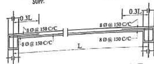
Details Of R.C.C Roof Slab & Beam
