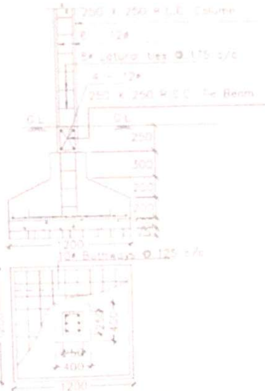
DETAILS OF R.C.C. COLUMN (SCALE - 1/20)
