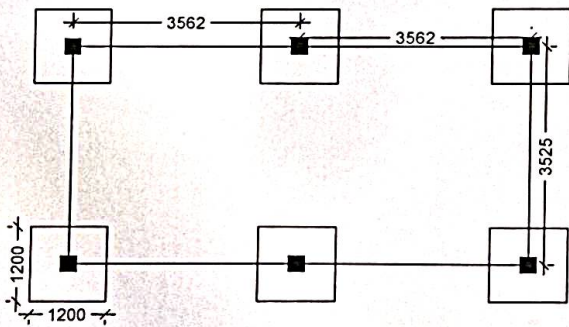
LAYOUT PLAN
