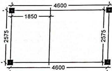
LAYOUT PLAN
