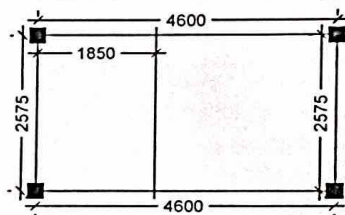
LAYOUT PLAN
