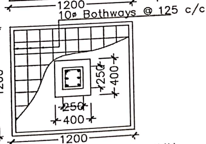
DETAILS OF R. C. C COLUMN (SCALE - 1 : 25)
