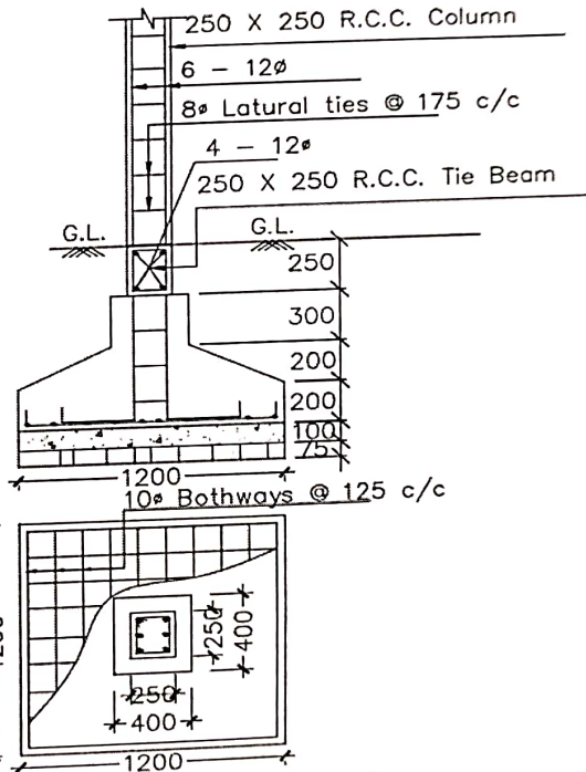
DETAILS OF R. C. C COLUMN (SCALE - 1 : 25)
