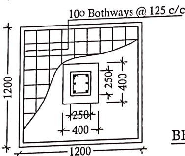
DETAILS OF R. C. C COLUMN (SCALE - 1:25)
