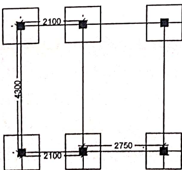
LAYOUT PLAN
