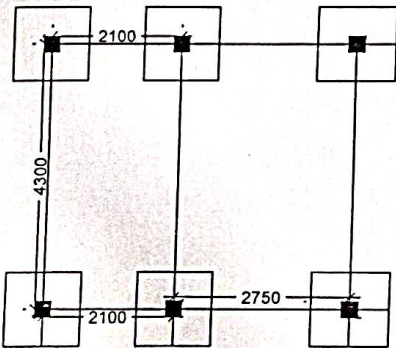
LAYOUT PLAN
