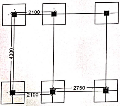
LAYOUT PLAN
