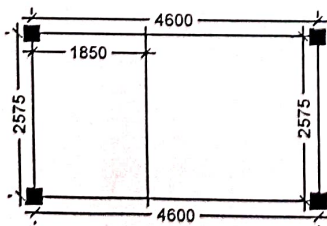
LAYOUT PLAN
