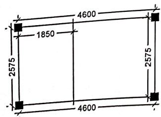
LAYOUT PLAN
