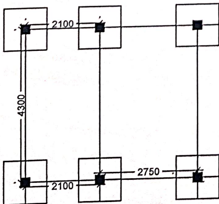
LAYOUT PLAN
