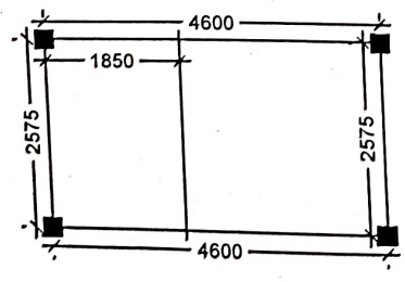
LAYOUT PLAN
