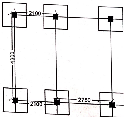
LAYOUT PLAN
