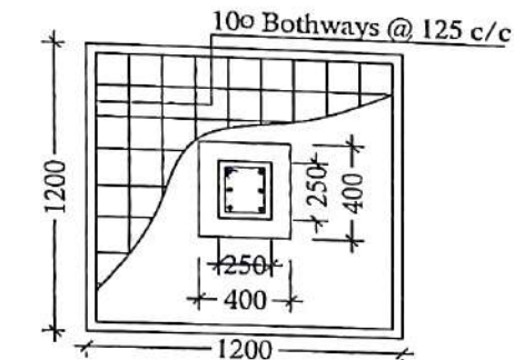
DETAILS OF R. C. C COLUMN (SCALE - 1 : 25)
