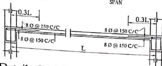
Details Of R.C.C Roof Slab & Beam (SCALE - 1 : 25)
