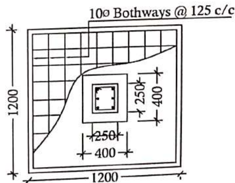
DETAILS OF R. C. C COLUMN (SCALE - 1 : 25)
