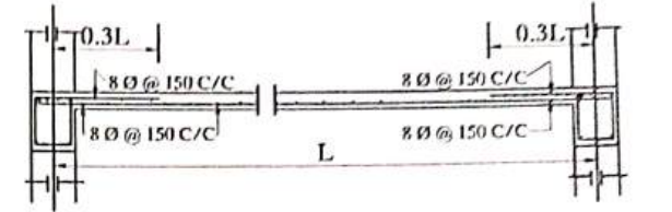
Details Of R.C.C Roof Slab & Beam
