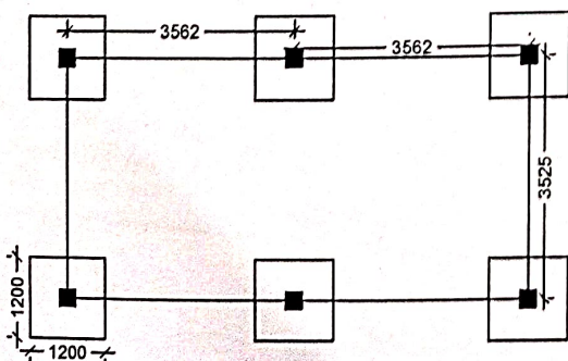
LAYOUT PLAN
