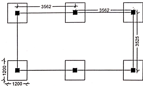
LAYOUT PLAN
