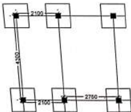
LAYOUT PLAN
