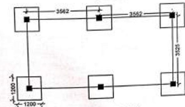
LAYOUT PLAN
