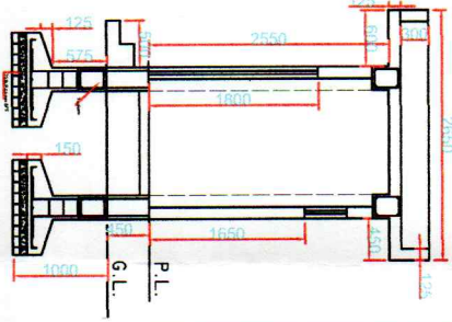
Typical Beam Details
