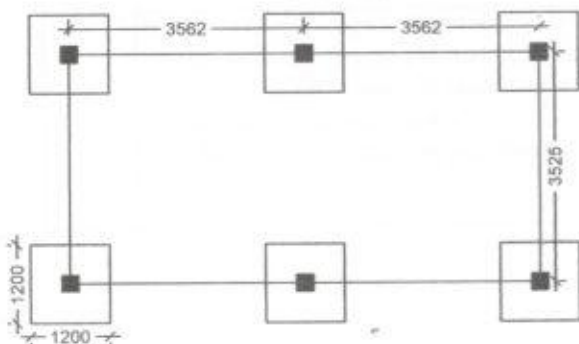
LAYOUT PLAN
