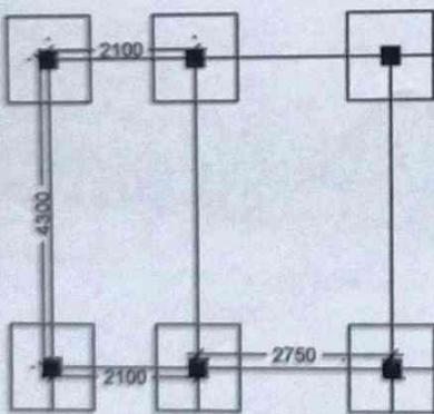
LAYOUT PLAN
