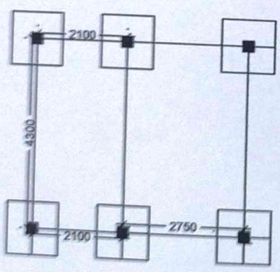
LAYOUT PLAN
