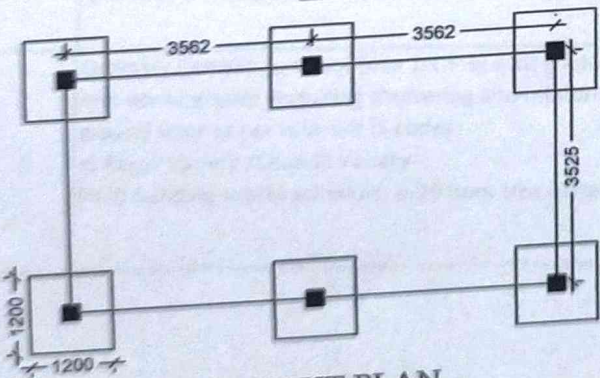
LAYOUT PLAN
